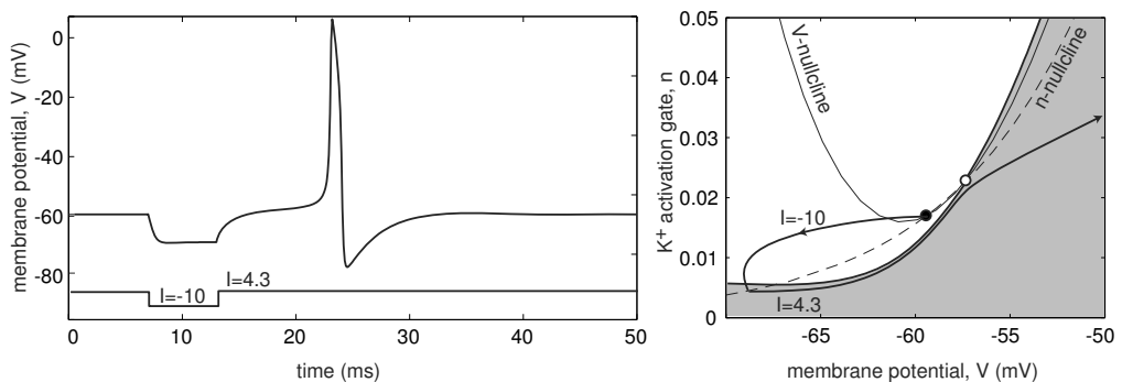
Figure 7.40: Postinhibitory spike of an integrator neuron near Bogdanov-Takens bifurcation; see Fig.7.39.
