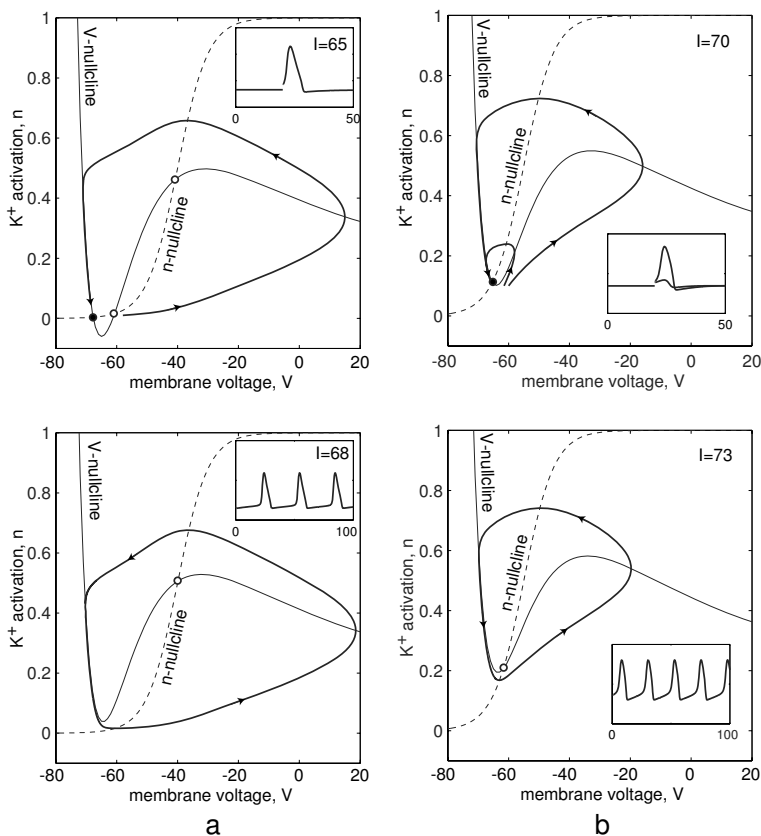
Figure 5.12: Possible intersections of nullclines in the I_K + I_{Kir} -model. Parameters: E_K = -80 mV, g_{Kir} = 20 , g_K = 2 . Instantaneous I_{Kir} with V_{1/2} = -80 mV and k = -12 . Slower I_K with k = 5 , \tau(V) = 5 ms, and V_{1/2} = -40 mV (in a) or V_{1/2} = -55 mV (in b).
