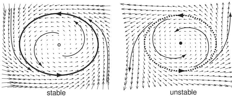
Figure 4.9: Limit cycles (periodic orbits).
