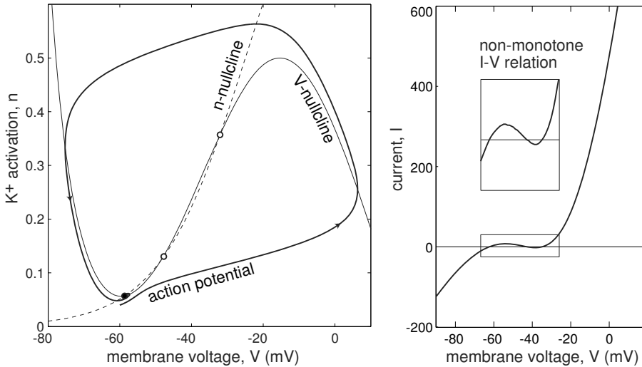
Figure 6.52: exercise 8: This I_{Na,p}+I_K -model has a non-monotonic I-V relation, yet the resting state becomes unstable via Andronov-Hopf bifurcation before disappearing via saddle-node bifurcation. Parameters are as in Fig.4.1a, except that E_{leak} = -78 mV and n_{\infty}(V) has k = 12 mV.
