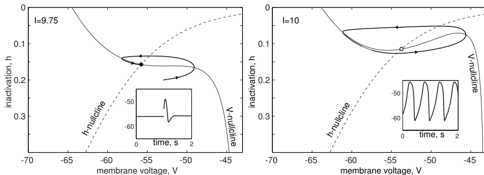
Figure 5.10: Resting and sustained subthreshold oscillations in the I_h + I_{K_{ir}} -model. Parameters: E_K = -80 mV, E_h = -43 mV, E_L = -50 mV, g_{K_{ir}} = 4 , g_h = 0.5 , g_L = 0.44 . The h-current is the same as in section 5.1.4, except V_{1/2} = -65 mV. Instantaneous I_{K_{ir}} has V_{1/2} = -76 mV and k = -11 .
