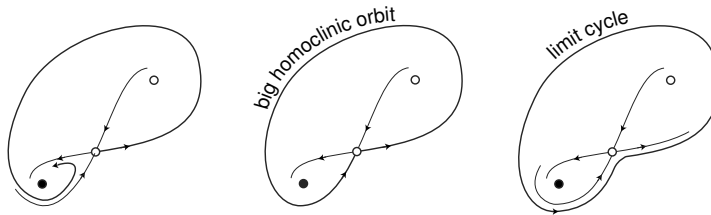
Figure 6.31: Big saddle homoclinic orbit bifurcation.
