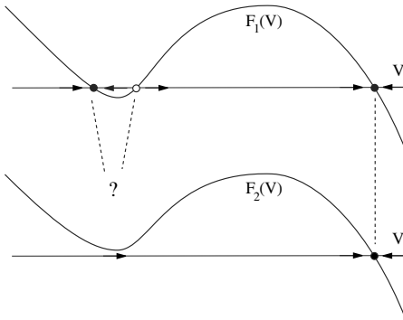
Figure 3.20: Two “seemingly alike” dynamical systems \dot{V} = F_1(V) and \dot{V} = F_2(V) are not topologically equivalent, hence they do not have qualitatively similar dynamics. (The first system has three equilibria, while the second system has only one.)
