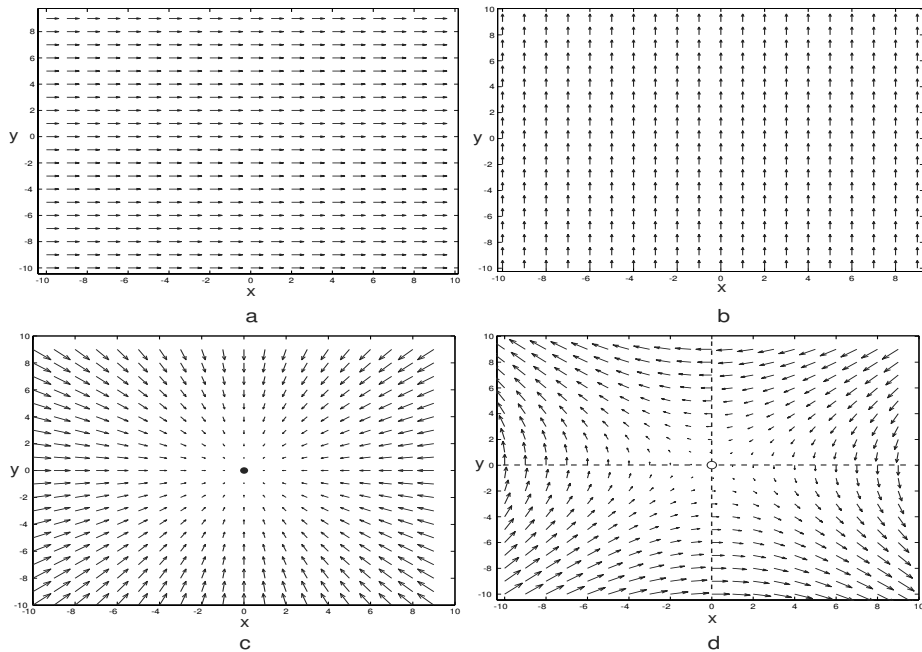
Figure 4.3: Examples of vector fields.
