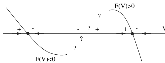
Figure 3.10: Two stable equilibrium points must be separated by at least one unstable equilibrium point because F(V) has to change the sign from “minus” to “plus”.
