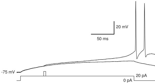
Figure 7.34: Long latencies and threshold crossing of layer 5 neuron recorded in vitro of rat motor cortex.
