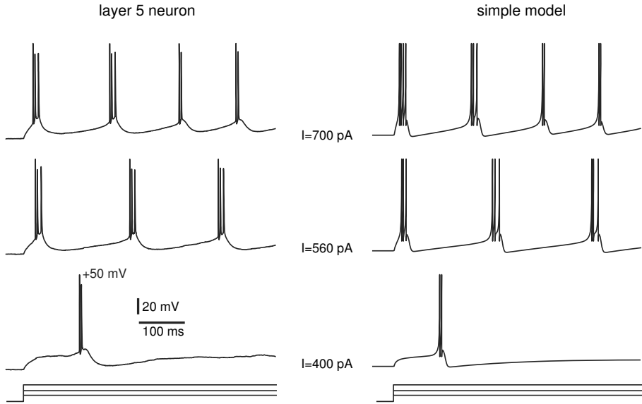
Figure 8.21: Comparison of in vitro recordings of an intrinsically bursting (IB) neuron (layer 5 of somatosensory cortex of a four-week-old rat at 35^{\circ}\text{C} ; data provided by Greg Stuart and Maarten Kole) with the two-compartment simple model. Soma: 150\dot{v} = 3(v + 70)(v + 45) + 50(v_d - v) - u + I , \dot{u} = 0.01\{5(v + 70) - u\} , if v \geq +50 , then v \leftarrow -52 , u \leftarrow u + 240 . Active dendrite: 30\dot{v}_d = (v_d + 50)^2 + 20(v - v_d) - u_d , \dot{u}_d = 3\{15(v_d + 50) - u_d\} , if v_d \geq +20 , then v_d \leftarrow -20 , u_d \leftarrow u_d + 500 .
