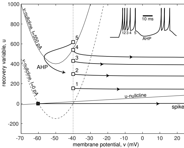
Figure 8.24: Phase portrait of the simple model in Fig.8.23 exhibiting CH firing pattern.
