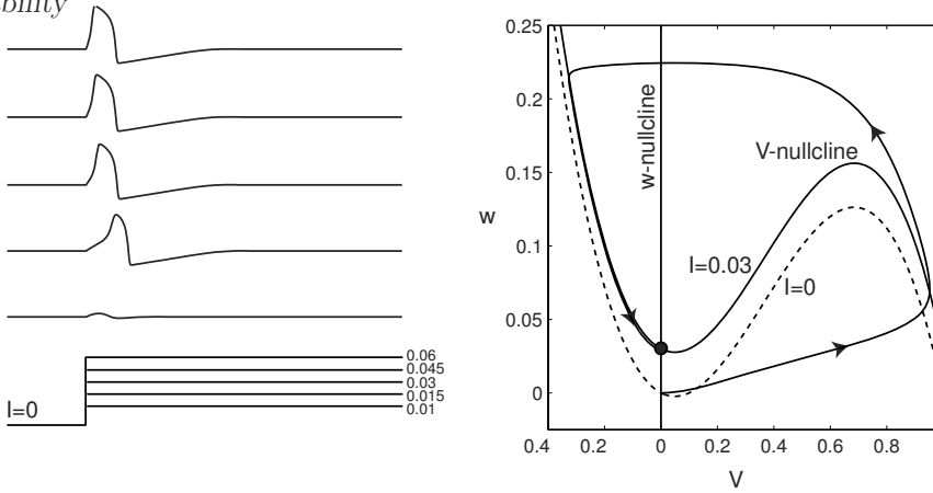
Figure 7.8: Class 3 excitability in FitzHugh-Nagumo model (4.11, 4.12) with a = 0.1, b = 0.01, c = 0 . The model fires a single spike for any pulse of current.
