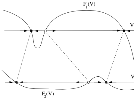
Figure 3.19: Two “seemingly different” dynamical systems, \dot{V} = F_1(V) and \dot{V} = F_2(V) , are topologically equivalent. Hence they have qualitatively similar dynamics.
