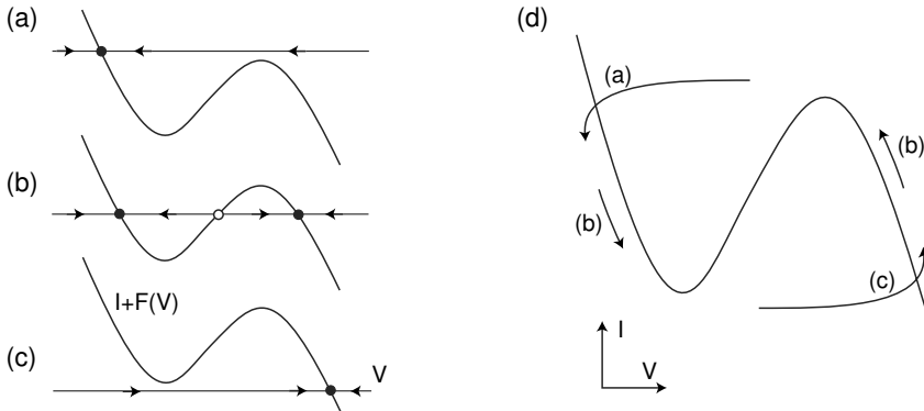
Figure 3.17: Bistability and hysteresis loop as I changes.
