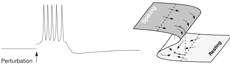
Figure 9.18: Burst excitability: a perturbation causes a burst of spikes.
