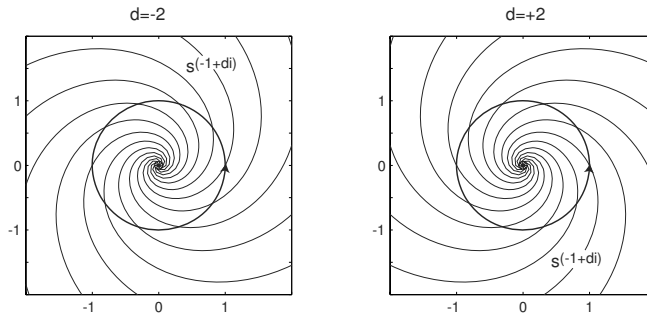
Figure 10.45: Isochrons of the Andronov-Hopf oscillator; see exercise 2.
