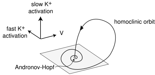
Figure S.28: Codimension-2 Shilnikov-Hopf bifurcation.
