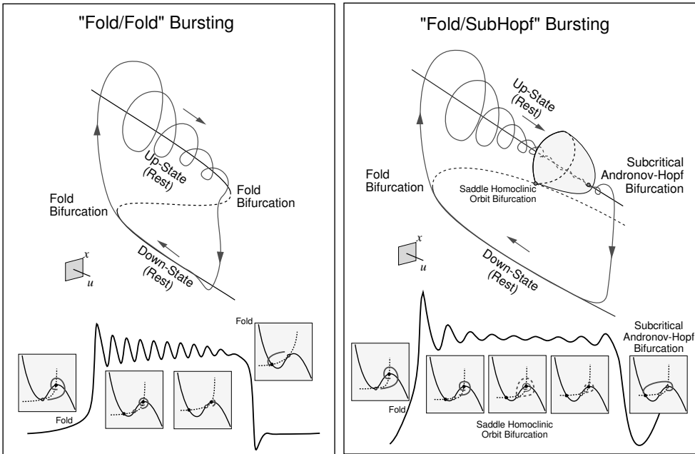
Figure 9.61: Two examples of point-point (not fast-slow) bursters. (Modified from Izhikevich 2000a.)
