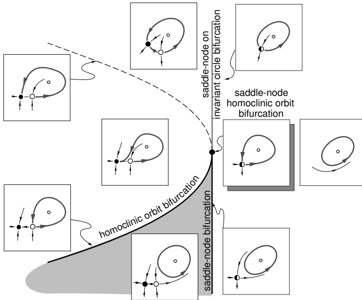
Figure 6.45: Unfolding of saddle-node homoclinic orbit bifurcation.
