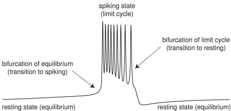
Figure 9.22: Two important bifurcations associated with fast-slow bursting.
