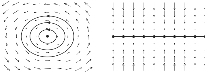
Figure 4.13: Neutrally stable equilibria. Some trajectories neither converge to nor diverge from the equilibria.
