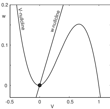
Figure 9.57: Rebound bursting in the FitzHugh-Nagumo oscillator; see exercise 4.
