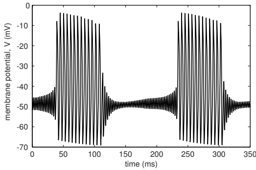
Figure 9.59: Bursting in the I_{Na,p}+I_K+I_{Na,slow} -model; see exercise 10.
