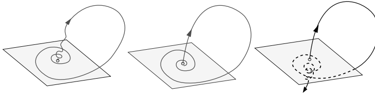
Saddle-Focus Homoclinic Orbit Bifurcation
