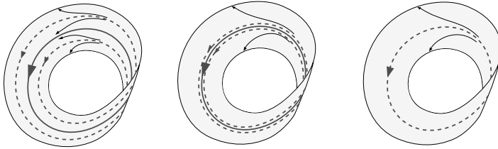
Subcritical Flip Bifurcation
