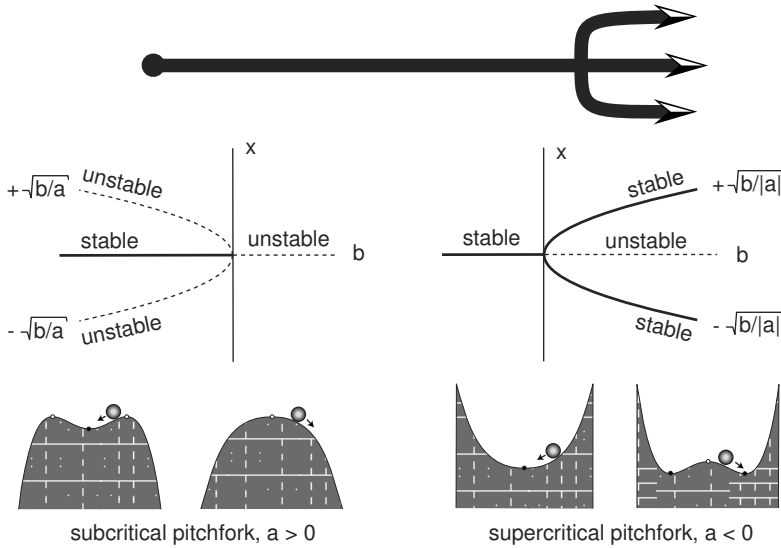
Figure 6.36: Pitchfork bifurcation diagrams.
