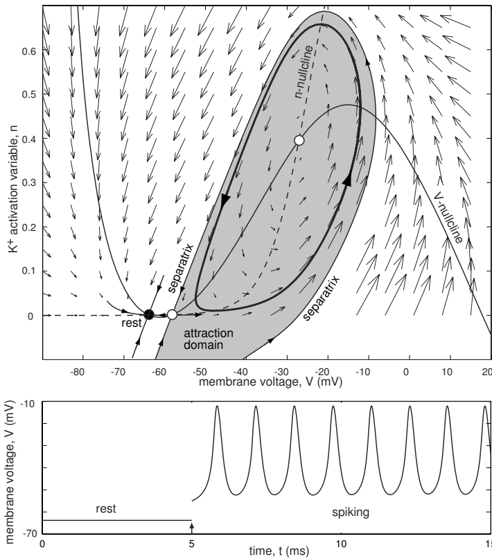
Figure 4.23: Bistability of rest and spiking states in the I_{Na,P} + I_K -model (4.1, 4.2) with high-threshold fast ( \tau(V) = 0.152 ) K^+ current and I = 3 . A brief strong pulse of current (arrow at t = 5 ms) brings the state vector of the system into the attraction domain of the stable limit cycle.
