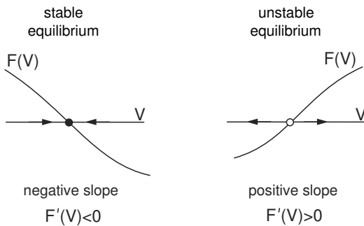
Figure 3.9: The sign of the slope, \lambda = F'(V) , determines the stability of the equilibrium.
