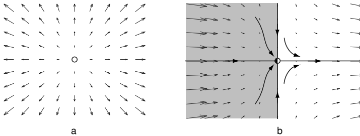
Figure 4.14: Unstable equilibria.
