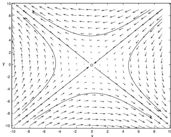
Figure 4.6: Representative trajectories of the two-dimensional system (4.3, 4.4).
