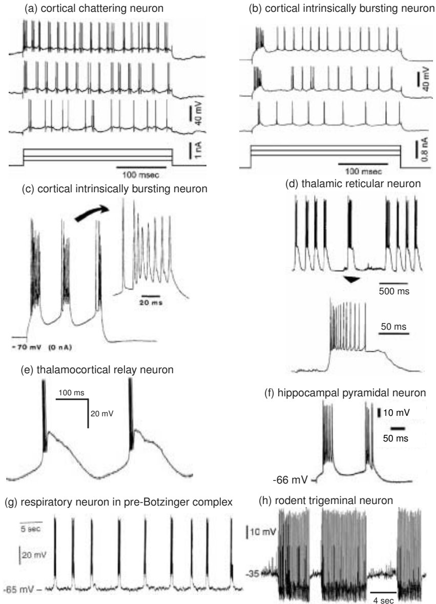
Figure 9.1: Examples of intrinsic bursters. (a) and (b) cat primary visual cortical neurons (modified from Nowak et al. 2003). (c) cortical neuron in anesthetized cat (modified from Timofeev et al. 2000). (d) thalamic reticular (RE) neuron (modified from Steriade 2003). (e) Cat thalamocortical relay neuron (modified from McCormick and Pape 1990). (f) CA1 pyramidal neuron exhibiting grade II low-threshold bursting pattern (modified from Su et al. 2001). (g) respiratory neuron in the pre-Botzinger complex (modified from Butera et al. 1999). (h) Trigeminal interneuron from rat brainstem (modified from Del Negro et al. 1998).
