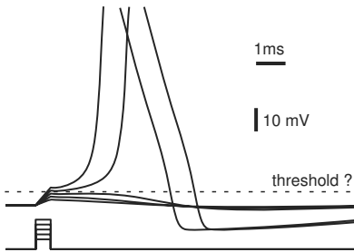
Figure 7.25: Finding the threshold in the Hodgkin-Huxley model.
