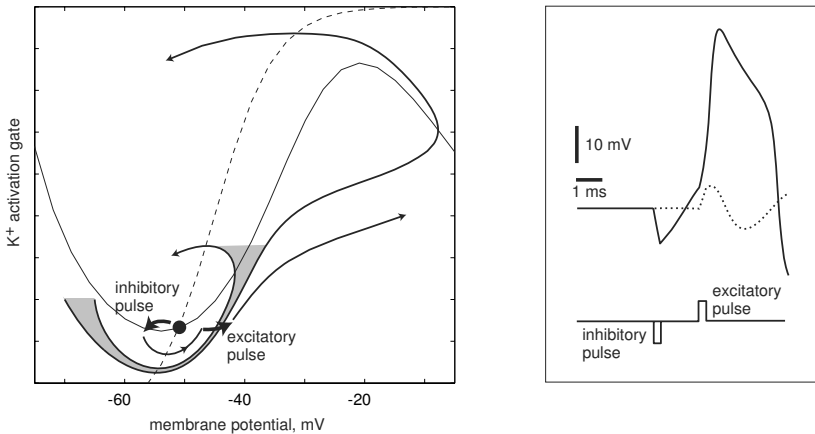
Figure 7.31: Postinhibitory facilitation: A subthreshold excitatory pulse can become suprathreshold if it is preceded by an inhibitory pulse.
