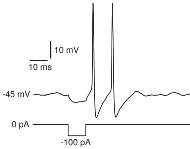
Figure 7.29: Rebound spikes in response to a brief hyperpolarizing pulse in a brainstem mesV neuron having fast subthreshold oscillations of membrane potential.
