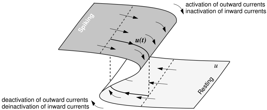
Figure 9.17: Hysteresis loop periodic bursting.
