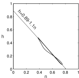
Figure 5.19: The relationship between n(t) and h(t) in the Hodgkin-Huxley model can be better described by h = 0.89 - 1.1n .
