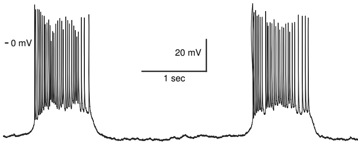
Figure 9.27: Putative “fold/homoclinic” bursting in a cell located in the pre-Botzinger complex of rat brain stem. (Data shared by Christopher A. Del Negro and Jack L. Feldman, Systems Neurobiology Laboratory, Department of Neurobiology, UCLA.)
