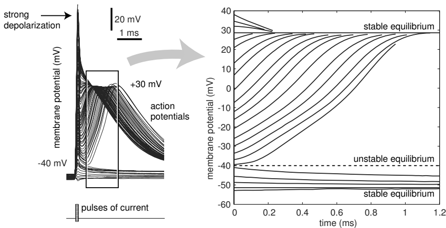
Figure 3.15: Upstroke dynamics of layer 5 pyramidal neuron in vitro (compare with the I_{\text{Na,p}} -model (3.5) in Fig.3.8b).
