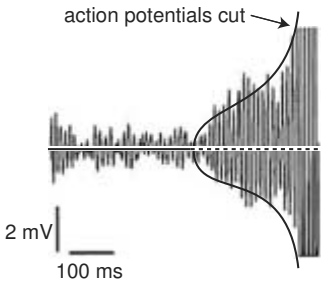
Figure 9.46: The conductance noise destabilizes the focus equilibrium in a mesencephalic V neuron before subcritical Andronov-Hopf bifurcation takes place, thereby giving an impression of a supercritical Andronov-Hopf bifurcation. (Data modified from Wu et al. 2001.)
