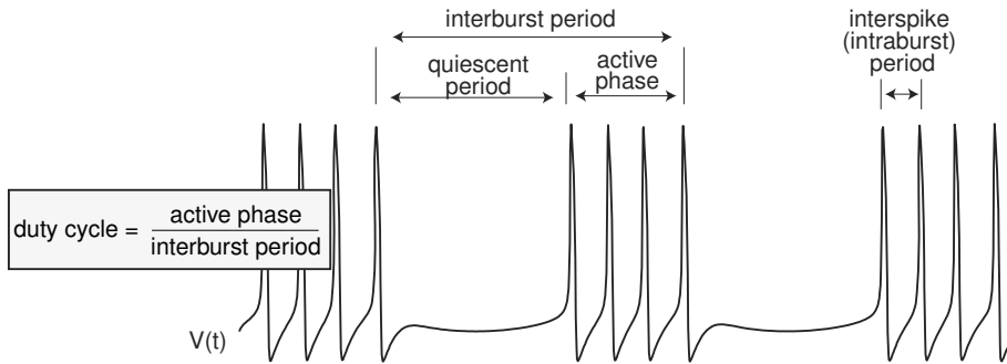
Figure 9.5: Basic characteristics of bursting dynamics.
