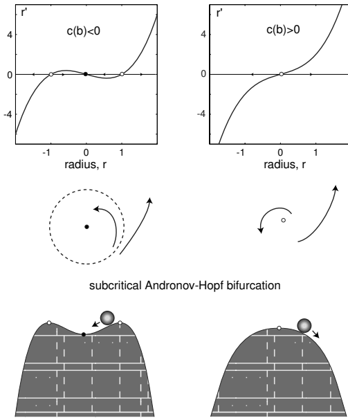
Figure 6.15: Subcritical Andronov-Hopf bifurcation in (6.8, 6.9) with c = \pm 1 and a = 1 .
