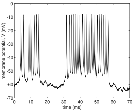
Figure 9.56: Bursting in a two-dimensional I_{Na,p}+I_K -model; see exercise 3.
