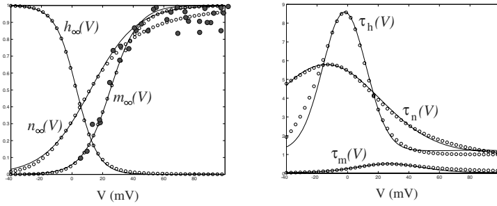
Figure S.1: Open dots : The steady-state (in)activation functions and voltage-sensitive time constants in the Hodgkin-Huxley model. Filled dots : steady-state Na + activation function m_\infty(V) in the squid giant axon (experimental results by Hodgkin and Huxley 1952, figure 8). Continuous curves : Approximations by Boltzmann and Gaussian functions. See exercise 4.
