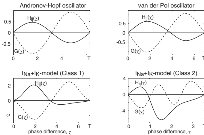
Figure 10.26: Solid curves. Functions H_{ij}(\chi) defined by (10.16) with the input g(x_i, x_j) = (x_{j1} - x_{i1}, 0) corresponding to electrical synapse via gap-junction. Dashed curves. Functions G(\chi) = H_{ji}(-\chi) - H_{ij}(\chi) . Parameters are as in Fig.10.3.
