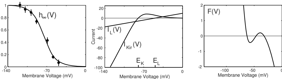
Figure 3.38: The I_{\text{Kir}} -model having injected current ( I ), leak current ( I_L ), and instantaneous \text{K}^+ inward rectifier current ( I_{\text{Kir}} ) and described by (3.11). Inactivation curve h_\infty(V) is modified from Wessel et al. (1999). Parameters: C = 1 , I = 6 , g_L = 0.2 , E_L = -50 , g_{\text{Kir}} = 2 , E_K = -80 , V_{1/2} = -76 , k = -12 (see Fig.2.20).
