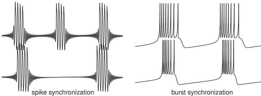
Figure 9.51: Various regimes of synchronization of bursters.
