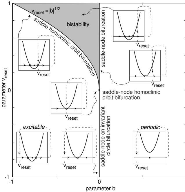
Figure 8.3: Bifurcation diagram of the quadratic integrate-and-fire neuron (8.2).
