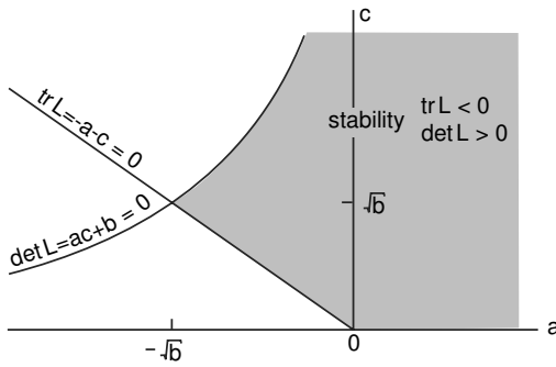
Figure 4.21: Stability diagram of the equilibrium (0,0) in the FitzHugh-Nagumo model (4.11,4.12).
