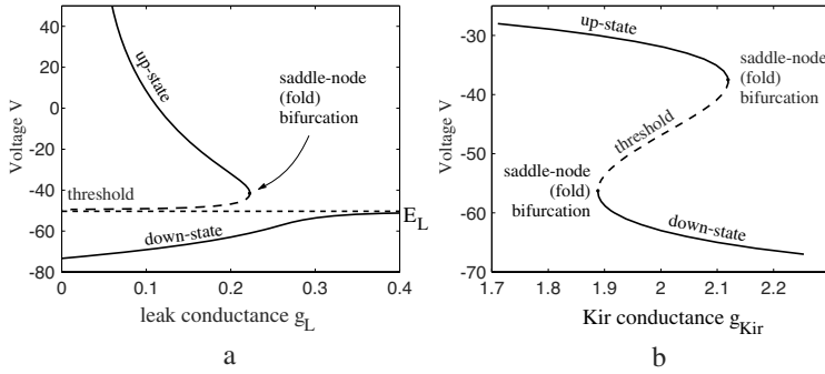
Figure S.10: Bifurcation diagrams of the I_{Kir} -model (3.11), I = 6 , with bifurcation parameters (a) g_L and (b) g_{Kir} (see chapter 3, exercise 12).
