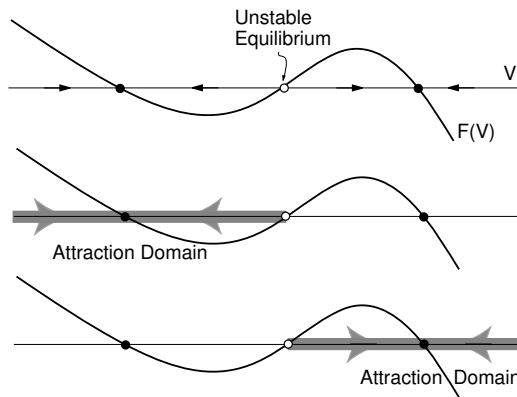
Figure 3.12: Two attraction domains in a one-dimensional system are separated by the unstable equilibrium.
