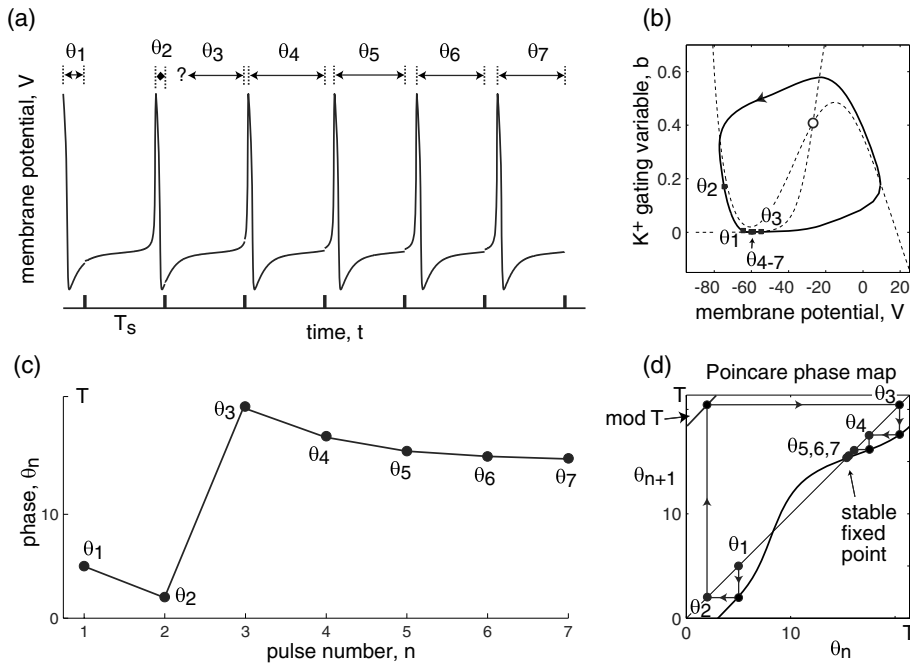
Figure 10.10: Description of synchronization of I_{Na} + I_K -oscillator in Fig.10.4, using Poincare phase map.
