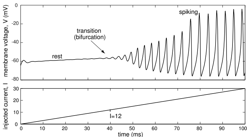
Figure 4.33: Transition from resting state to repetitive spiking in the I_{Na,p} + I_K -model with ramp injected current I ; see also Fig.4.34 (small-amplitude noise is added to the model to mask the slow passage effect). Note that the frequency of spiking is relatively constant for a wide range of injected current.
