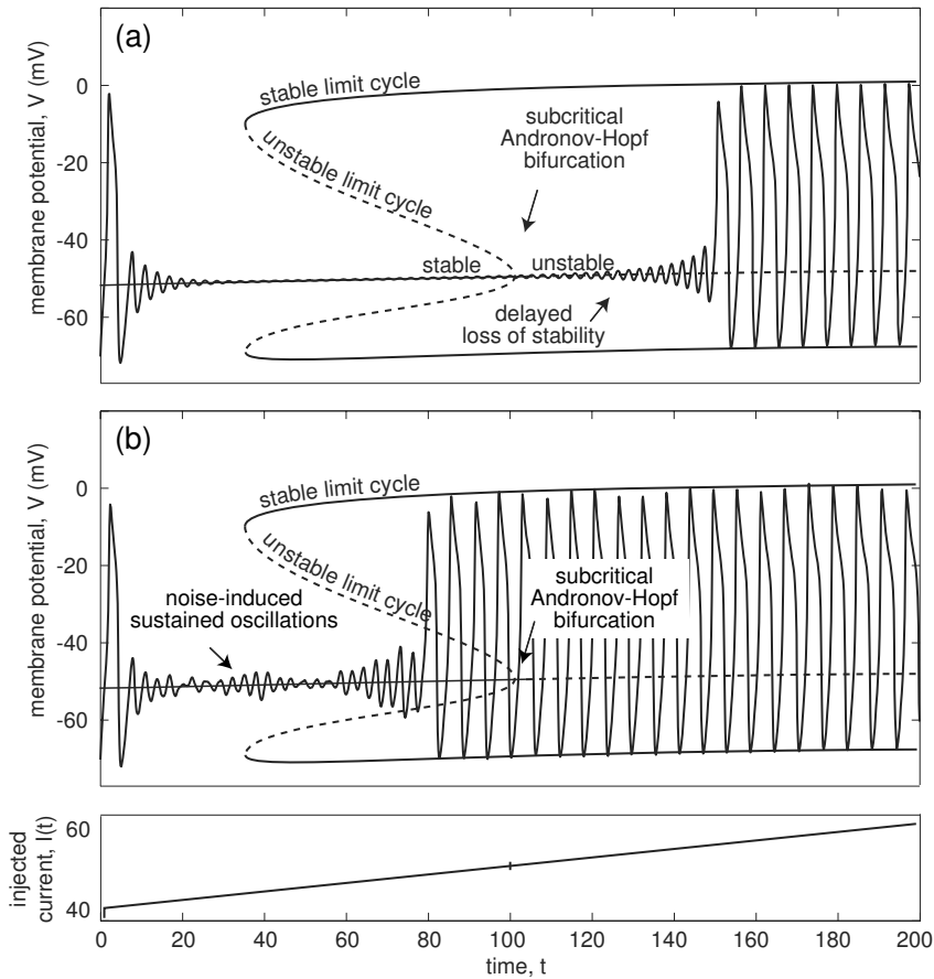
Figure 6.17: Delayed loss of stability (a) and noise-induced sustained oscillations (b) near subcritical Andronov-Hopf bifurcation. Shown are simulations of the I_{Na,p} + I_K -model with parameters as in Fig.6.16 and the same initial conditions. Small conductance noise is added in (b) to unmask oscillations.
